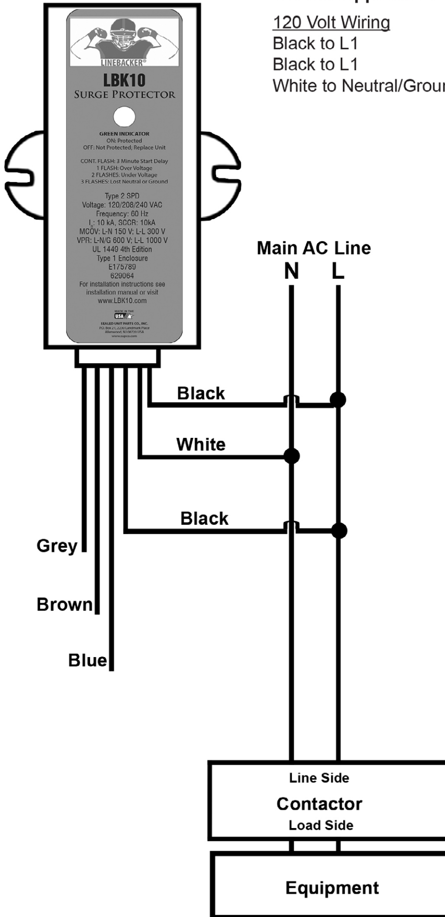
Figure 1B: 120VAC Application
